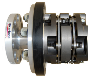
Flange Hub
