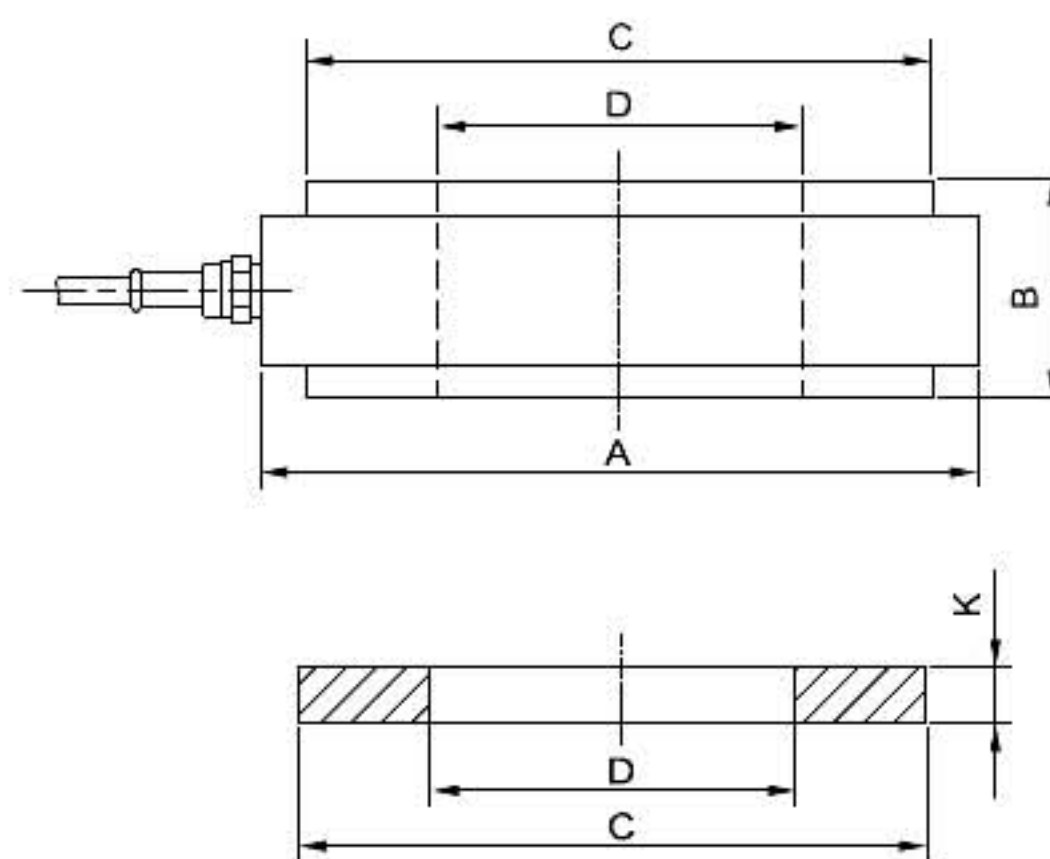
Washer (harden)
