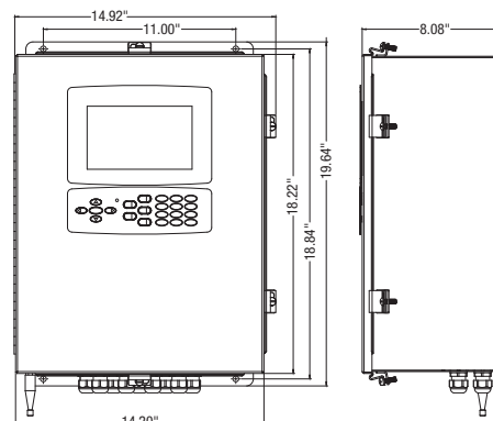
Wall Mount
