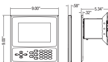
Panel Mount
